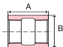
Fig. S3114CP & S3116CP - Full Coupling
