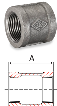
Fig. 33RL1 & 34RL1 – Right and Left Coupling
