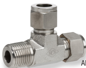
Fig. AMRT – Male Run Tee Double Ferrule
