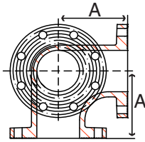
Fig. 38OE1 – 90° Side Outlet Elbow
