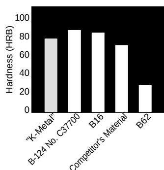
Fig. 2 Hardness Comparison
