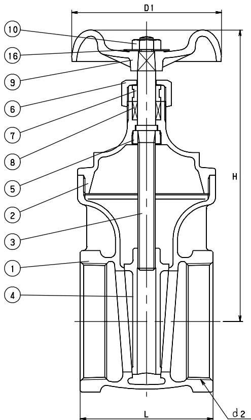
CODE # 27 (AKH) THREADED
