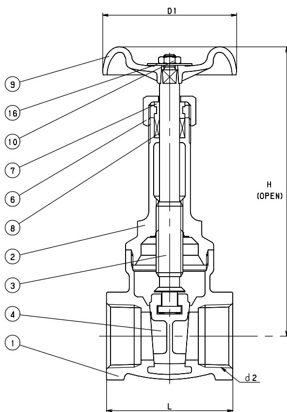
CODE # 25 (AK150L) THREADED
