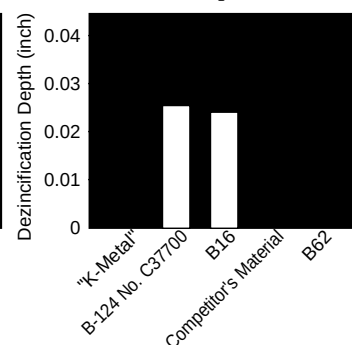
Fig. 4 Comparison of Dezincification Depth
