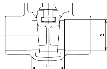
CODE # 45 (C150L) SOLDER*
