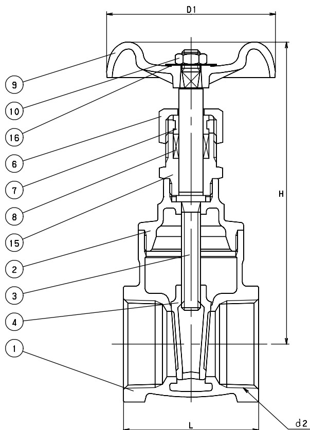
CODE # 46 (AK150E) THREADED
